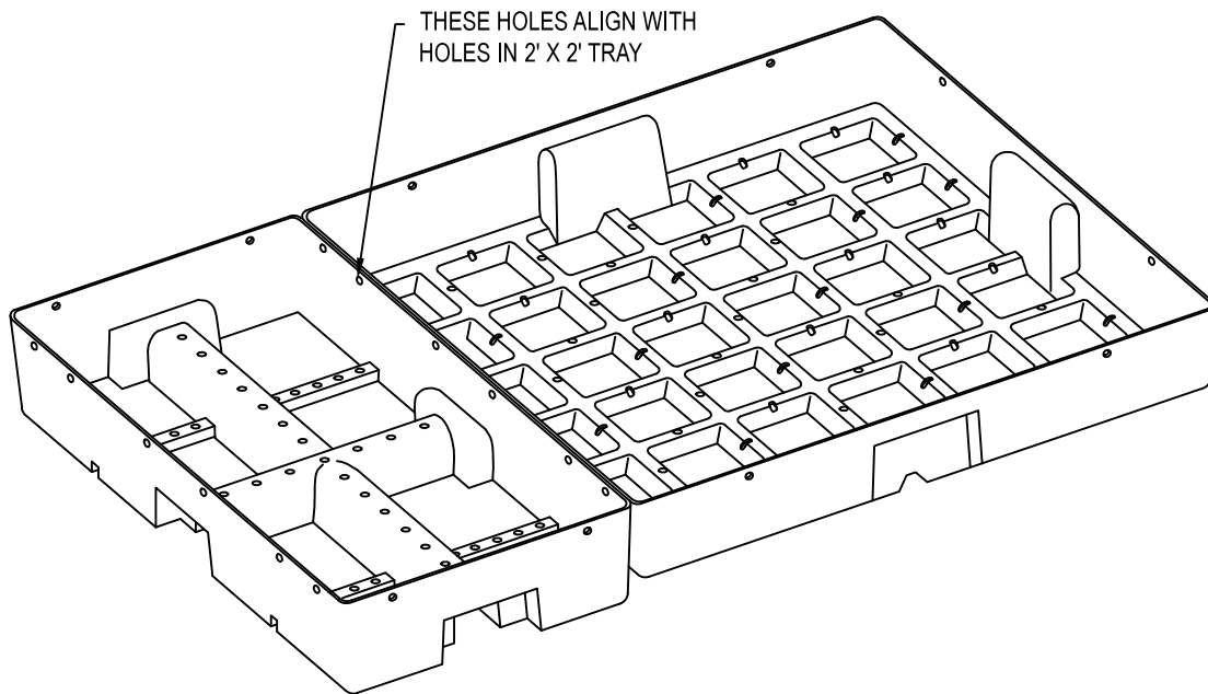
ISOMETRIC
