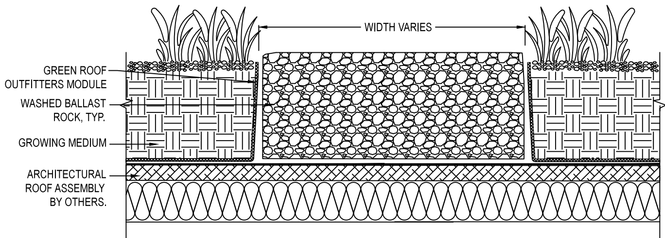
SECTION
